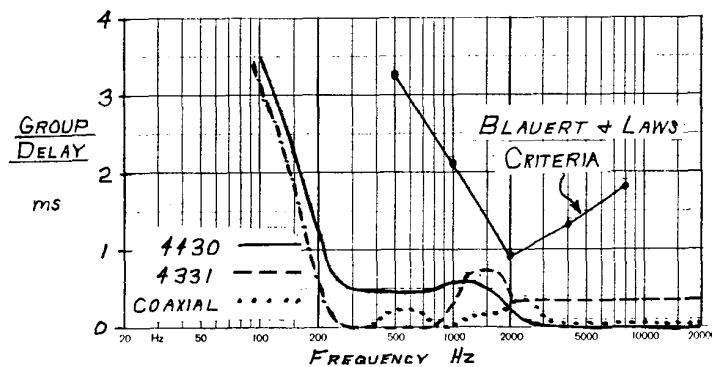
Fig. 19. Group delay versus Blauert and Laws criteria.
