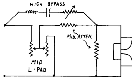
Fig. 7. High-end equalization network.
