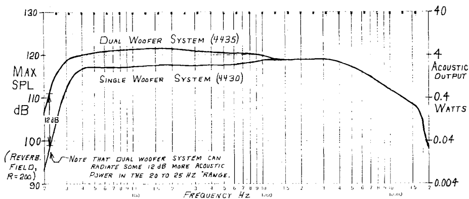
Fig. 20. Maximum continuous output (4430, 4435).
