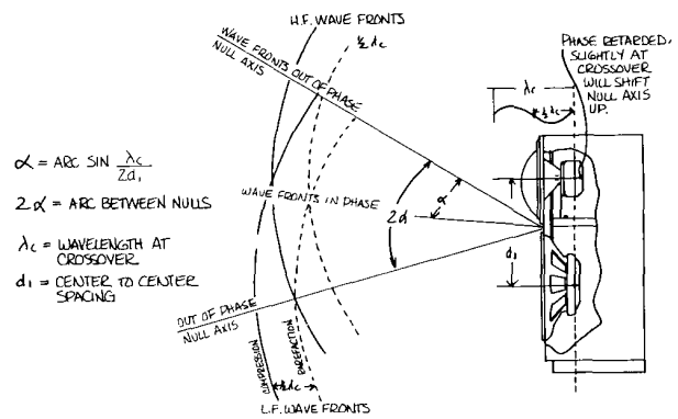
Fig. 10. Geometric causes of vertical off-axis response nulls.
