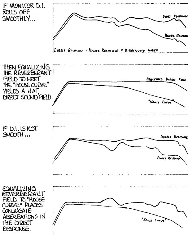
Fig. 21. Reverberant field equalization.
