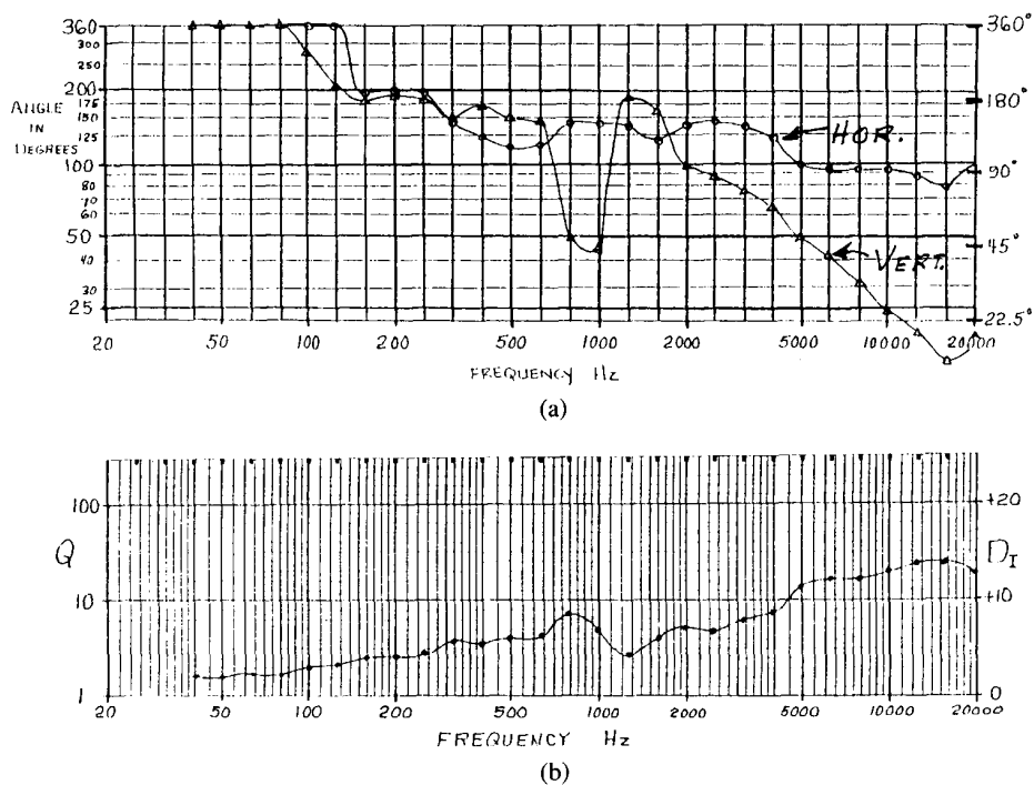
Fig. 12. Beamwidth and directivity index of two-way monitor (JBL 4331) using a 380 mm woofer and horn-lens assembly. (a) Beamwidth. (b) Directivity.
